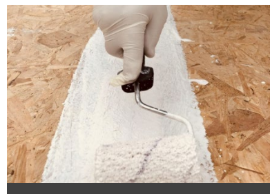
Square edge OSB3 joints reinforced with primer and taping mat
